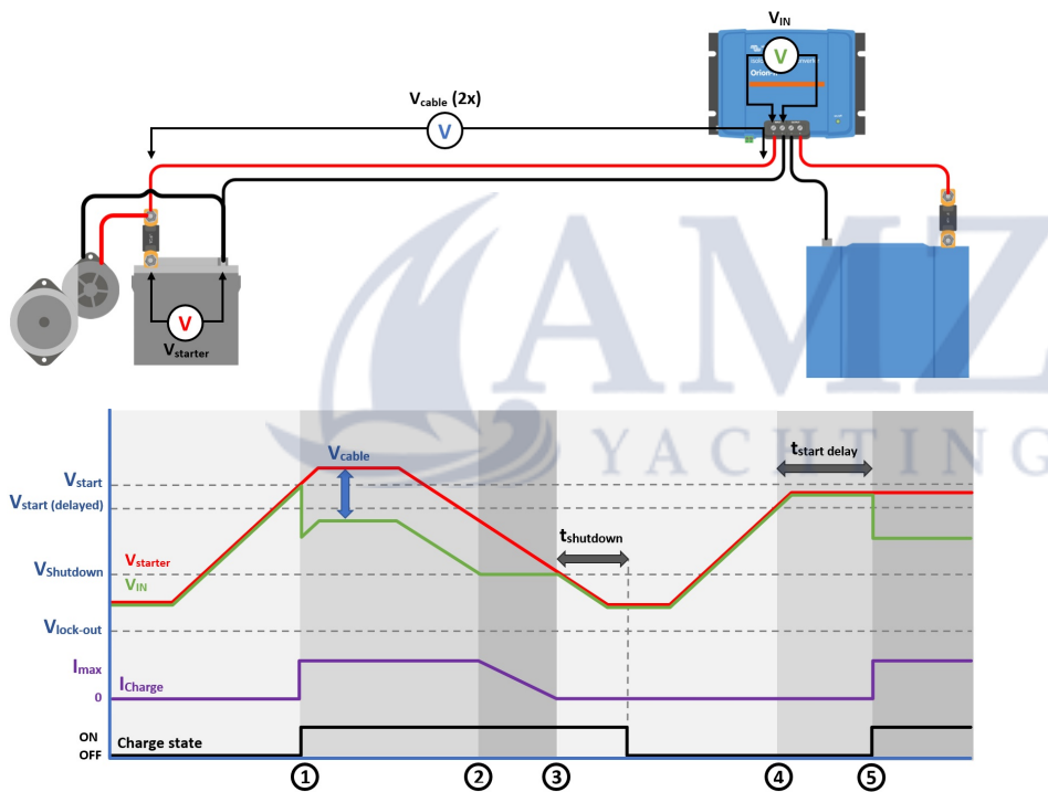
Figure 8: Engine shutdown detection sequence
